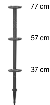
870084 ERDSPIESS GROUND SPIKE
